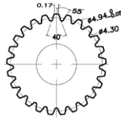
25T 5mm Output Shaft Spline
