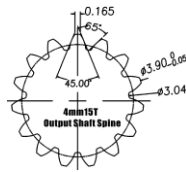
4mm 15T Output Shaft Spline
