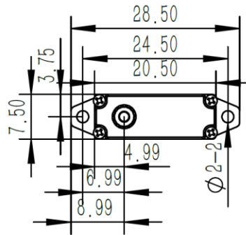
4mm 15T Output Shaft Spline
