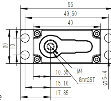
8mm25T Output Shaft Spline
