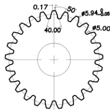
6mm25T Output Shaft Spline
