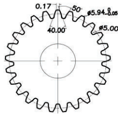
25T 6mm Output Shaft Spline
