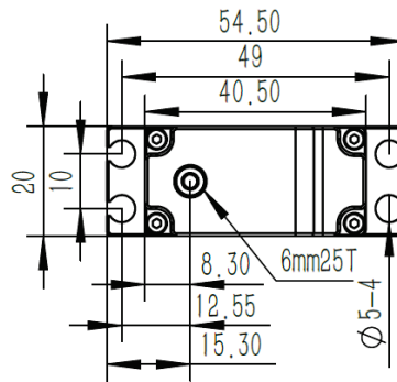
6mm 25T Output Shaft Spline
