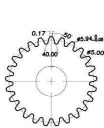
25T 6mm Output Shaft Spline
