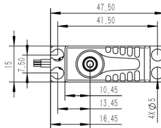
25T6mm Output Shaft Spline
