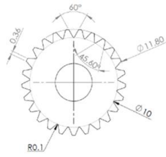
Output Shaft Spline (25T&12mm)
