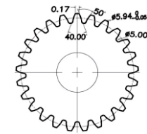
25T 6mm Output Shaft Spline
